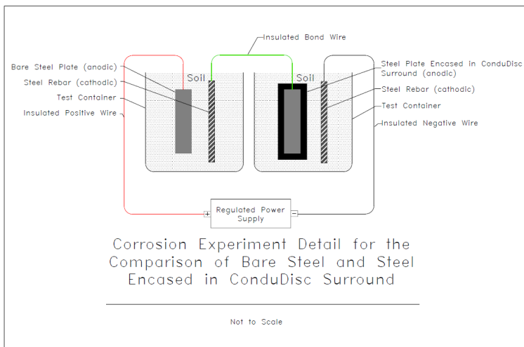
Figure 4: Schematics of the circuit configuration for each sample
