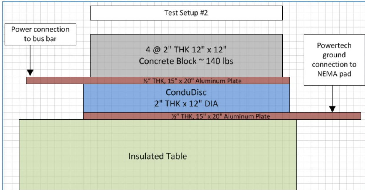
Figure #3: ConduDisc™, Test Setup #2
