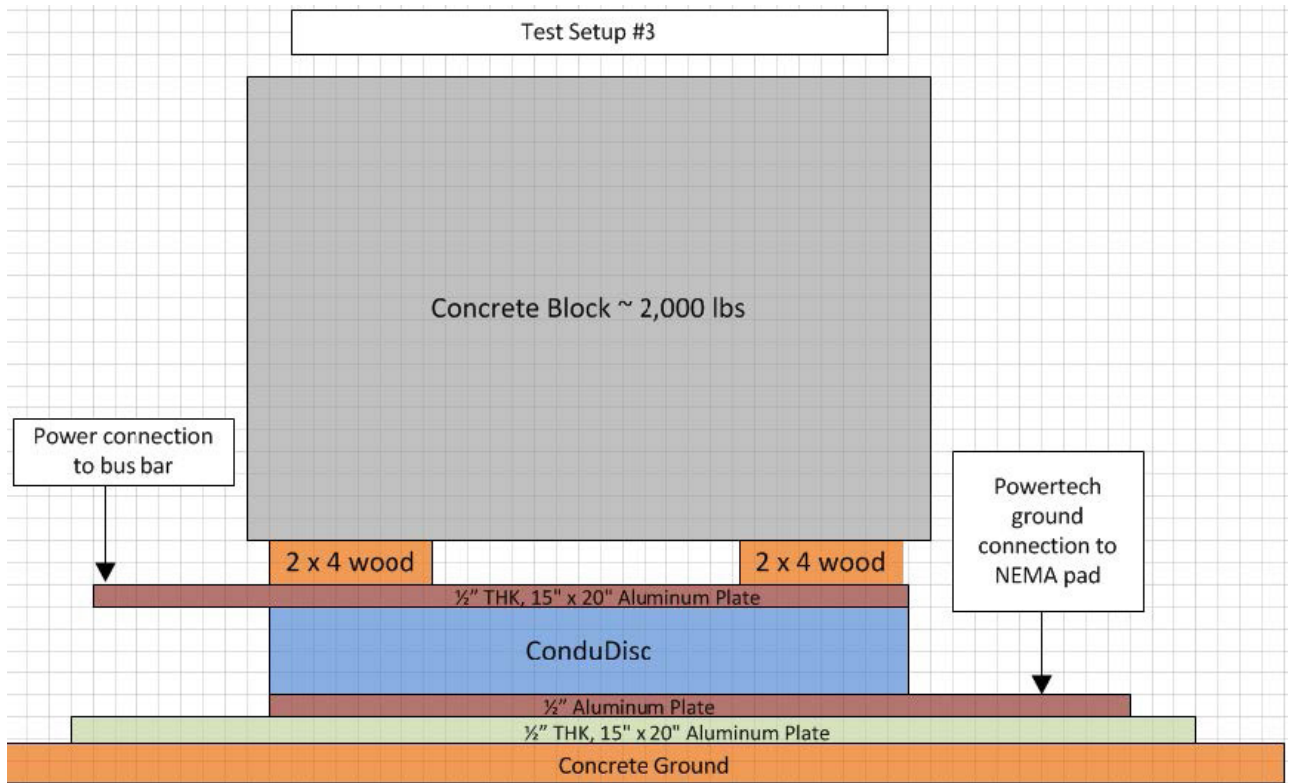
Figure 4: ConduDisc, Test Setup #3
