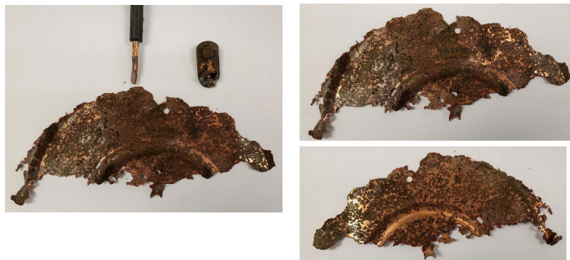
Figure 11: Blackburn GP-100 Copper Grounding Plate, After Experiment
