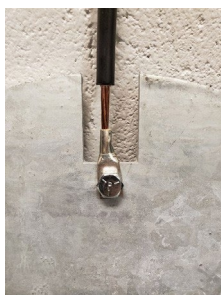
Figure 2: Copper Compression Connector Attachment to the Galvanized Steel Grounding Plate (left and middle) and the ConduDisc Inner Plate (right)
