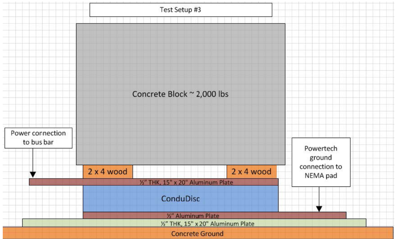
Figure 4: ConduDisc, Test Setup #3
