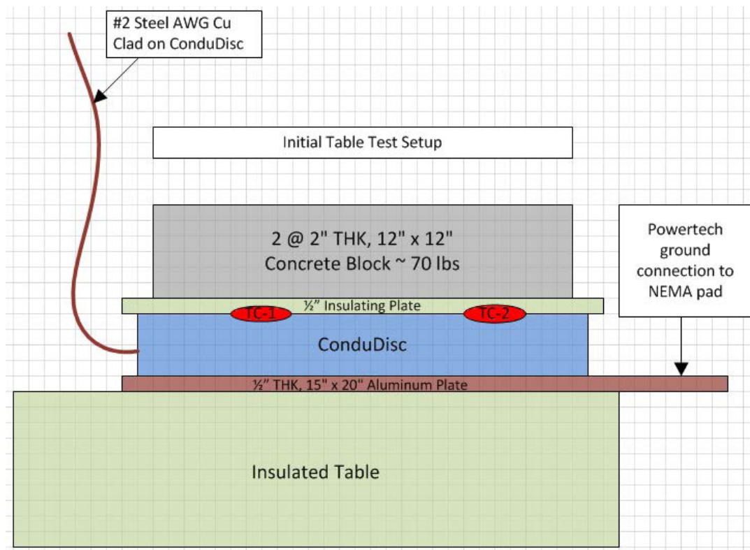
Figure 2: ConduDisc, Test Setup #1
