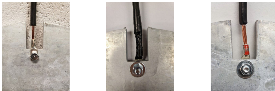
Figure 2: Copper Compression Connector Attachment to the Galvanized Steel Grounding Plate (left and middle) and the ConduDisc Inner Plate (right)
