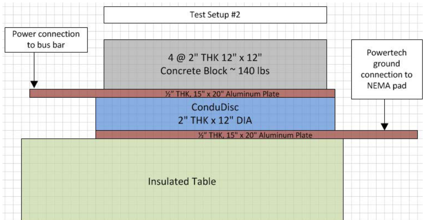
Figure 3: ConduDisc, Test Setup #2
